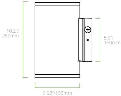
6" 2 LIGHT (CWSWP62)
