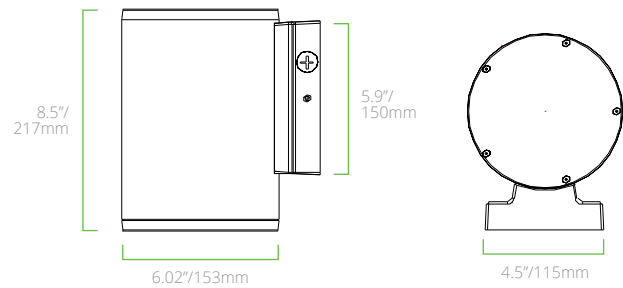
6" 1 LIGHT (CWSWP61)
