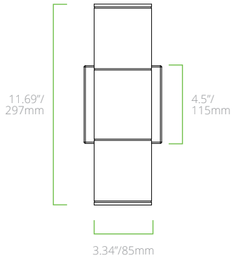
4" 2 LIGHT (CWSWP42)
