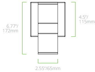
3" 1 LIGHT (CWSW31)
