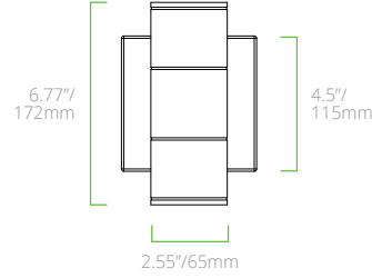
3" 2 LIGHT (CWSW32)
