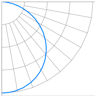
SLM24-62 / C5 (Typical performance @ 4000K)
