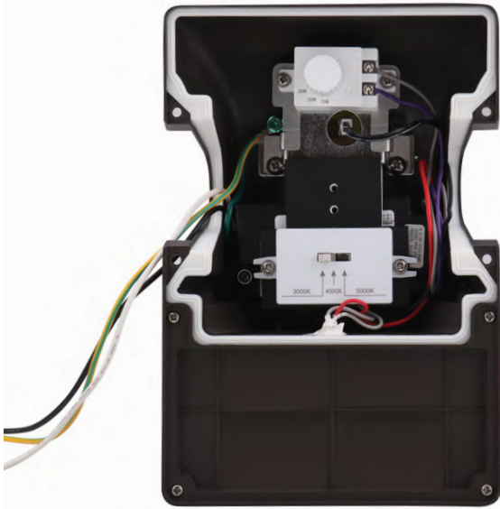
PHOTOCELL CONNECTED
