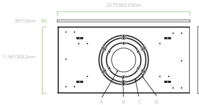
DL-NCPTG NEW CONSTRUCTION PLATE T-GRID
