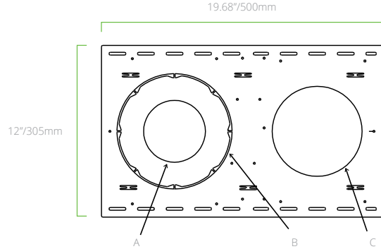
DL-NCPSJ NEW CONSTRUCTION PLATE STUD/JOIST
