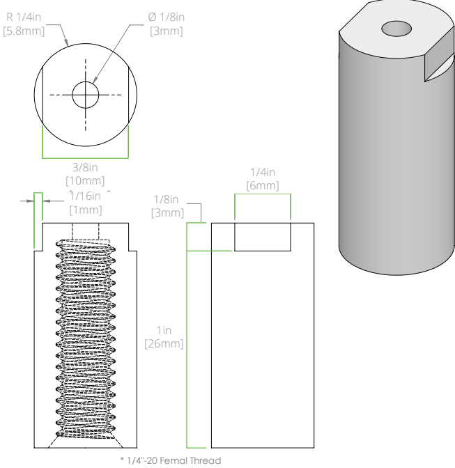
CABLE COUPLER
