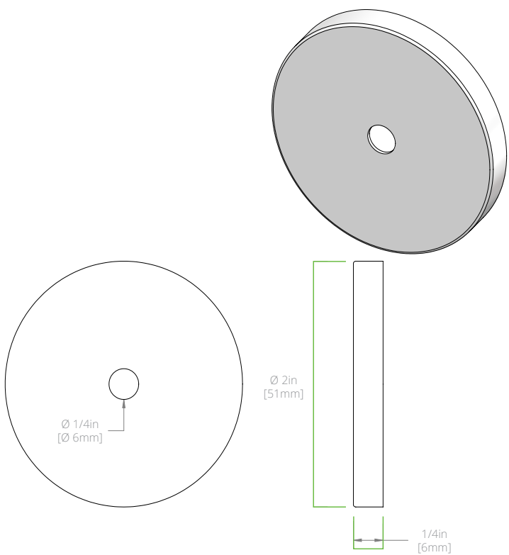
ROUND CANOPY
