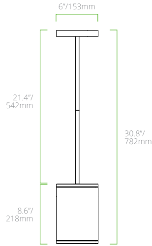
PENDANT MOUNT (CSMWP61 WITH PENDANT)
