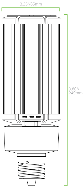
45W & 54W - EX39 HIGH VOLTAGE
