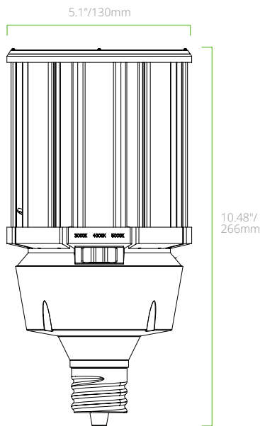
100W - EX39 HIGH VOLTAGE
