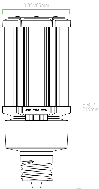
36W - EX39 HIGH VOLTAGE
