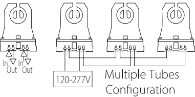
Non-Shunted Tombstones (lamp holders)
