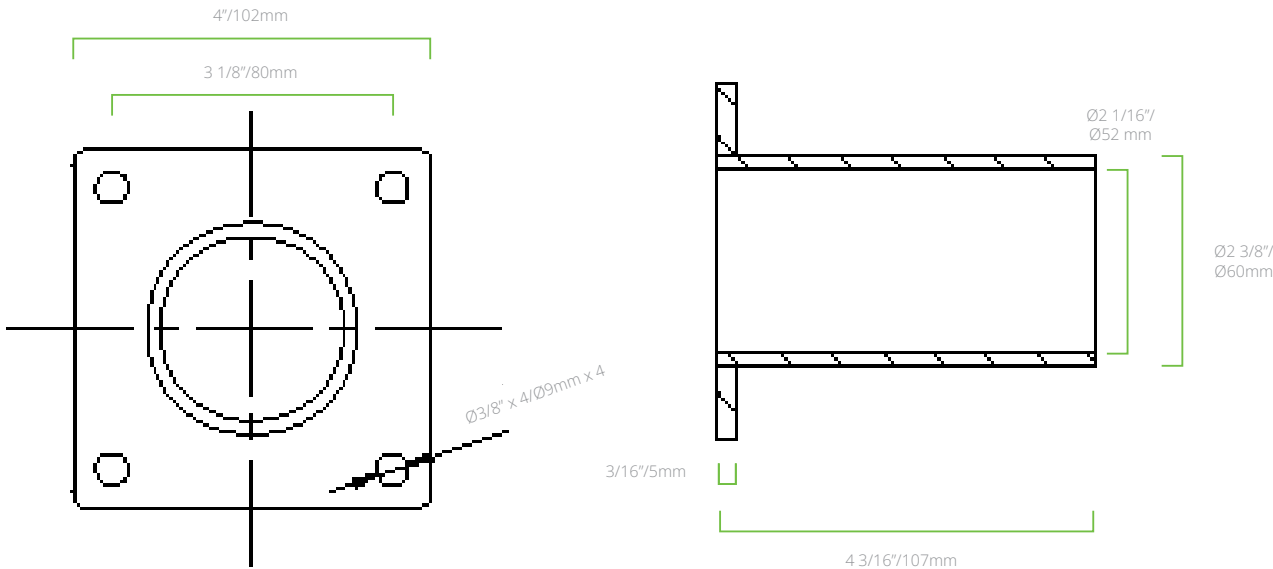
WB1-ST-BZ Weight: 2.1 lbs/0.9 kg
