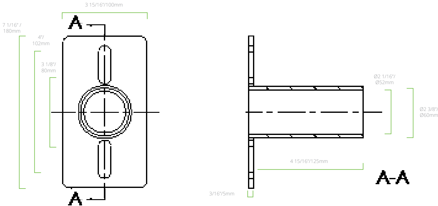
WB1-RT-BZ Weight: 2.8 lbs/1.3 kg
