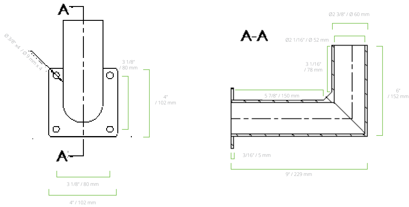
WB1-90RT-BZ Weight: 5.0 lbs / 2.3 kg
