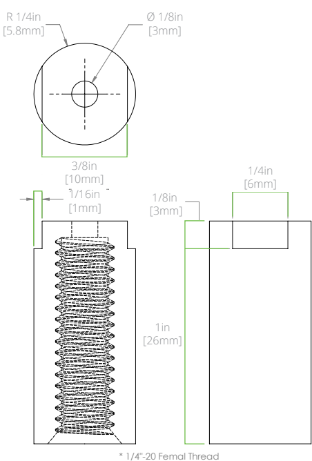
CABLE COUPLER
