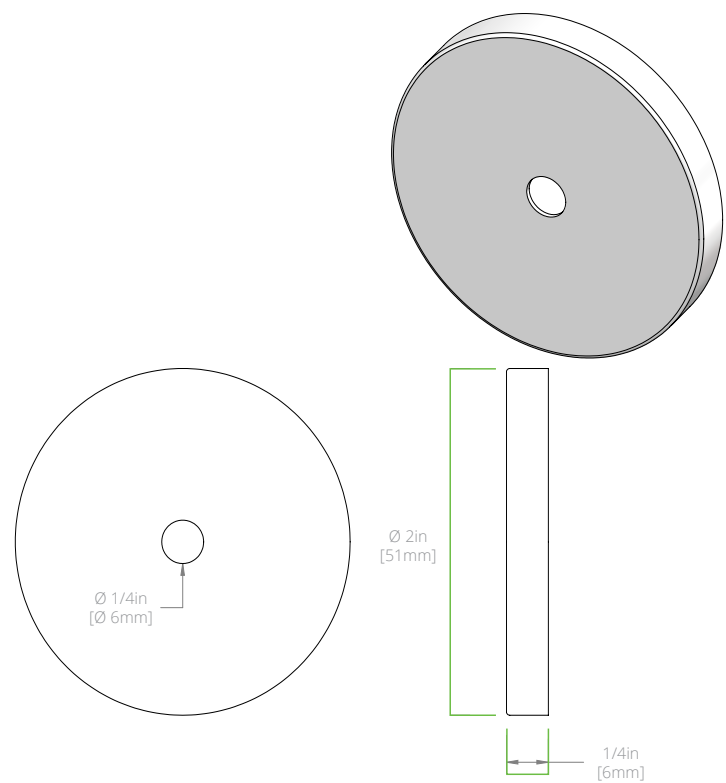
ROUND CANOPY
