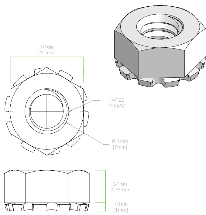
NUT W/ LOCK WASHER
