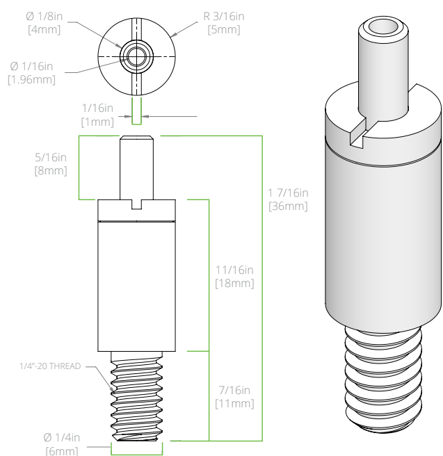
BOTTOM EXIT GRIPPER
