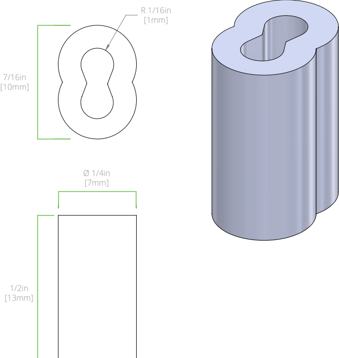
CABLE LOOP ADAPTER
